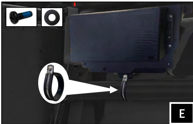
E. Mount the loop clamp to the bottom tube chassis and secure it to the amp tray using an included M4 x 12mm Phillips screw and washer.
